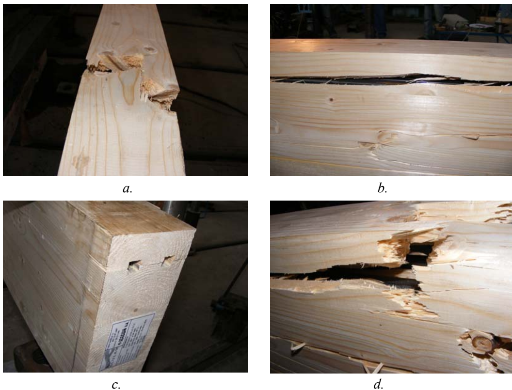
Fig. 8. Type of failure
