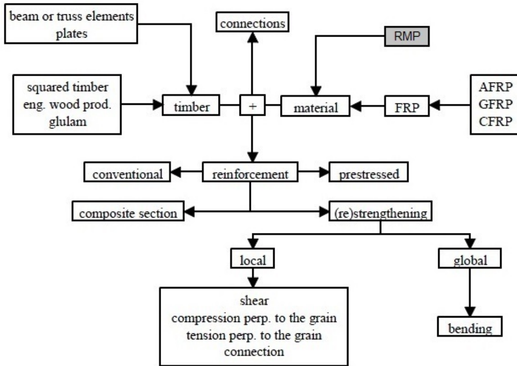
Fig. 1. Possibilities of using RMP in timber engineering
