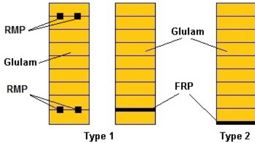
Fig. 3. Type of reinforced glulam beams cross section
