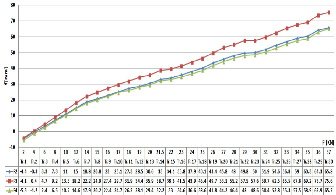
Fig. 7. Load-deflection curve of RMP double reinforced glulam
