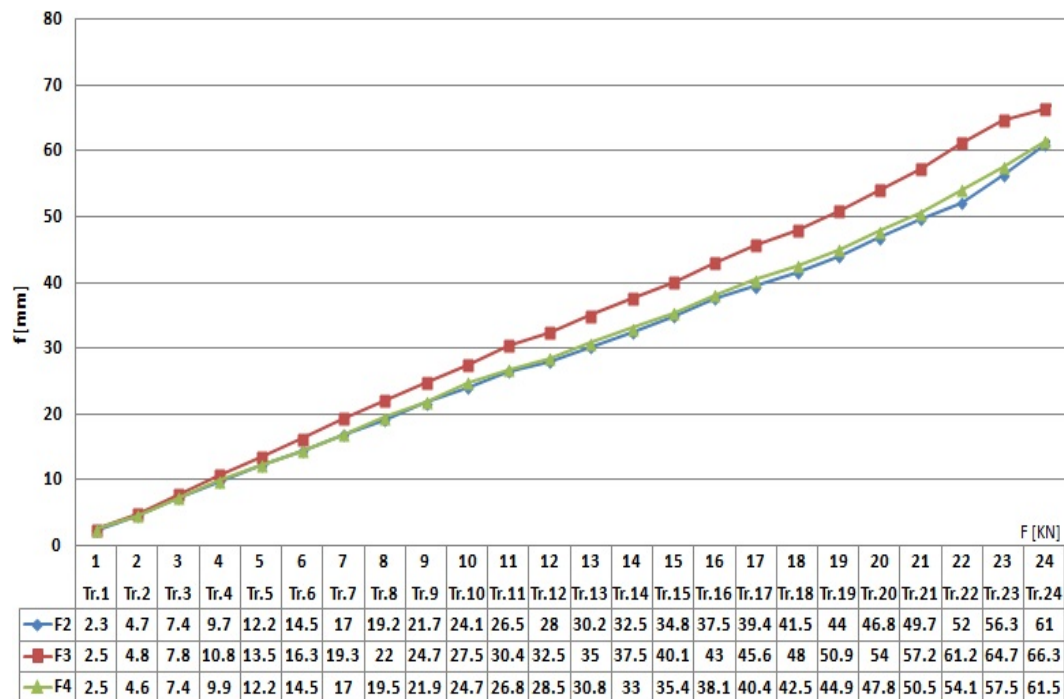
Fig. 6. Load-deflection curve of non-reinforced beam
